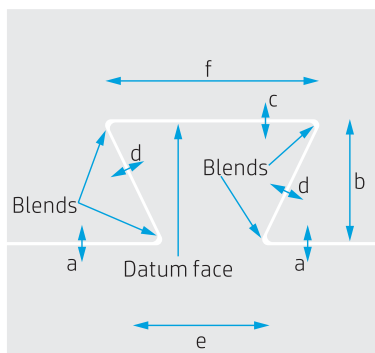
Figure 4: Dove/jigsaw design recommendations
