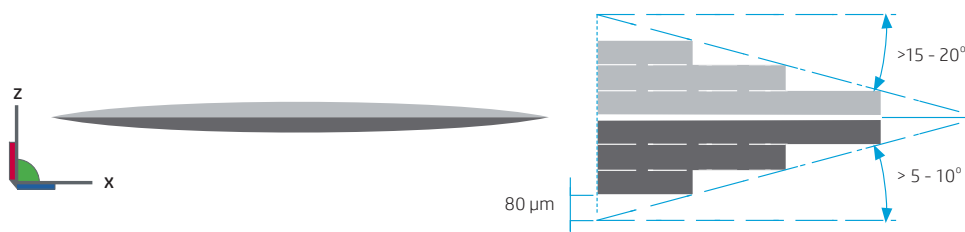
Figure 1: Stair-stepping effect
