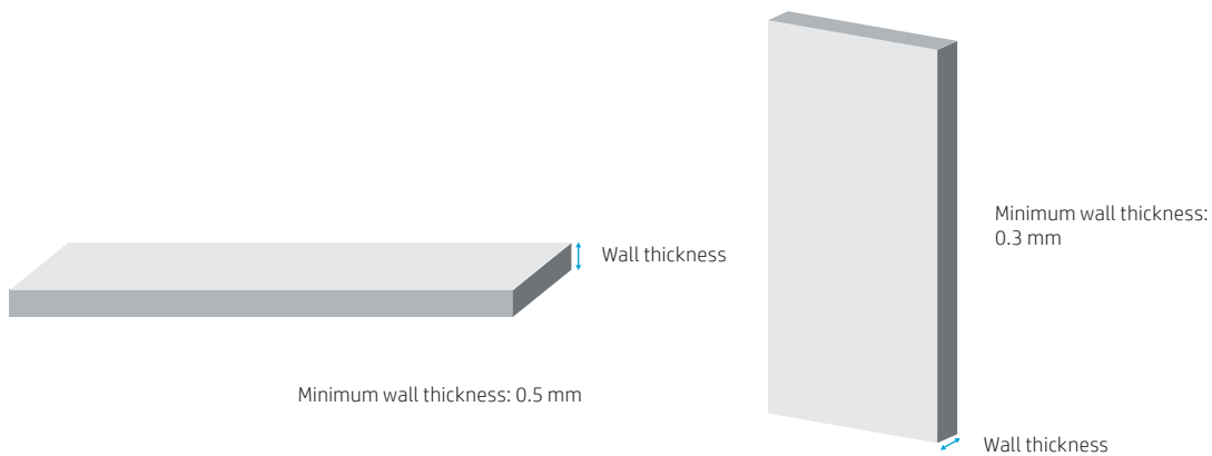
Figure 1. Minimum wall thickness
