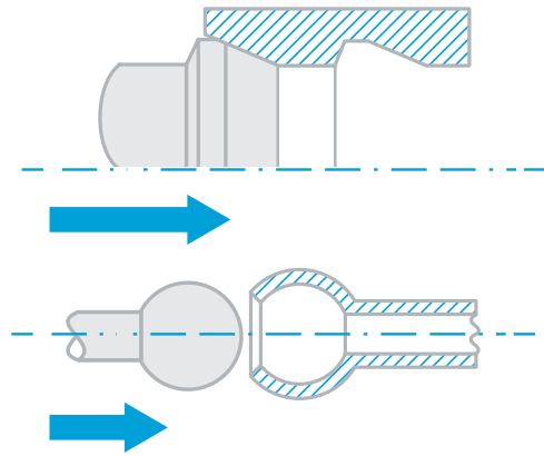
Figure 8. Annular snap-fit assembly operation
