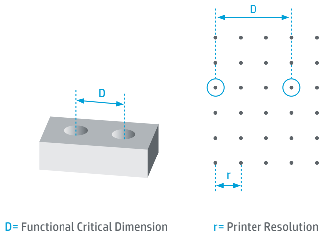
Figure 7. Printer resolution
