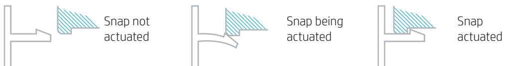
Figure 2. Cantilever snap-fit assembly operation
