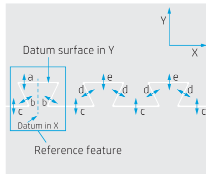
Figure 10: Multiple union features: Design recommendations
