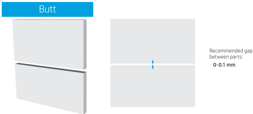
Figure 7: Butt design recommendations
