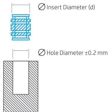
Figure 1: Hole diameter
