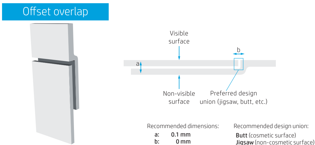
Figure 8: Offset overlap design recommendations
