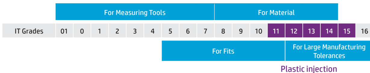
Figure 3: Plastic injection–equivalent IT Grades
