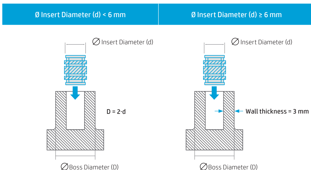
Figure 2: Boss diameter
