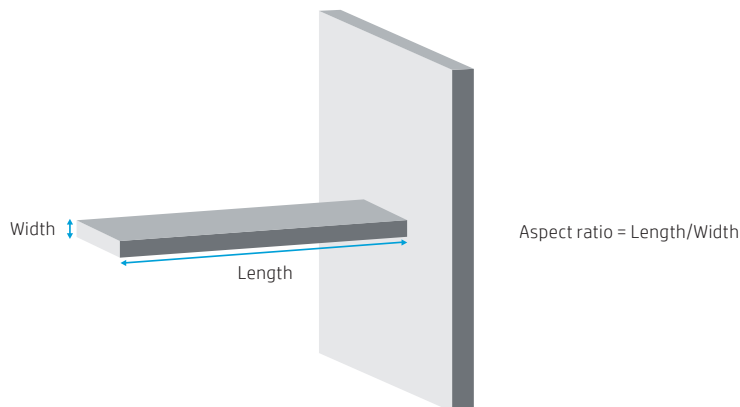
Figure 2. Cantilevers
